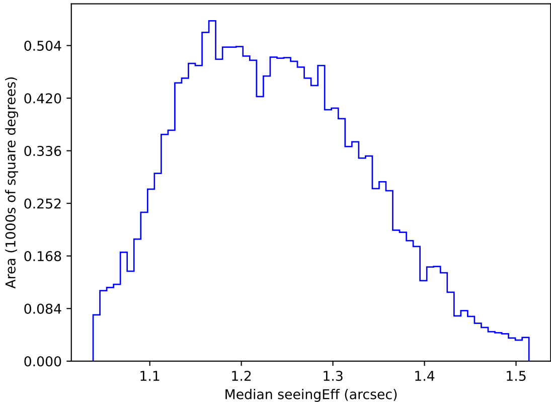
ddf_acor_sf20_lsf40_lsr50_v3.4_10yrs WFD u band: Median seeingEff
