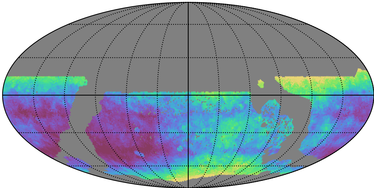
ddf_acor_sf20_lsf40_lsr50_v3.4_10yrs WFD i band: Median seeingEff
