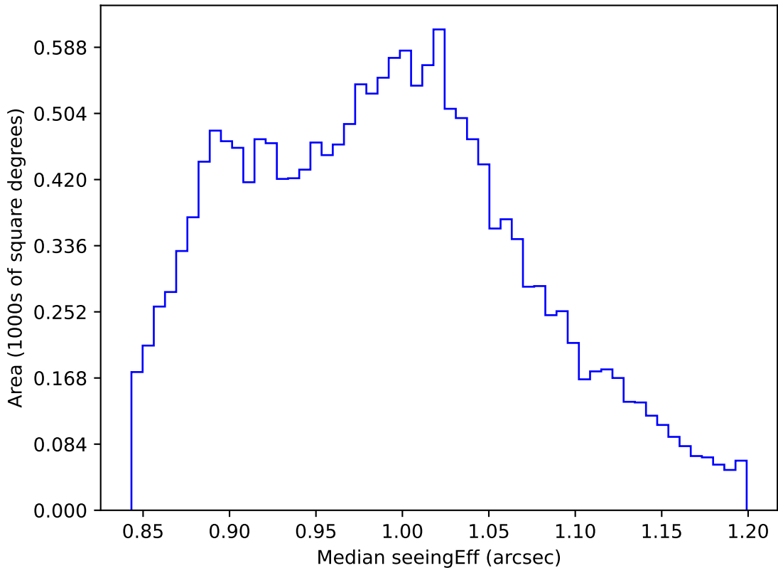
ddf_acor_sf20_lsf40_lsr50_v3.4_10yrs WFD i band: Median seeingEff
