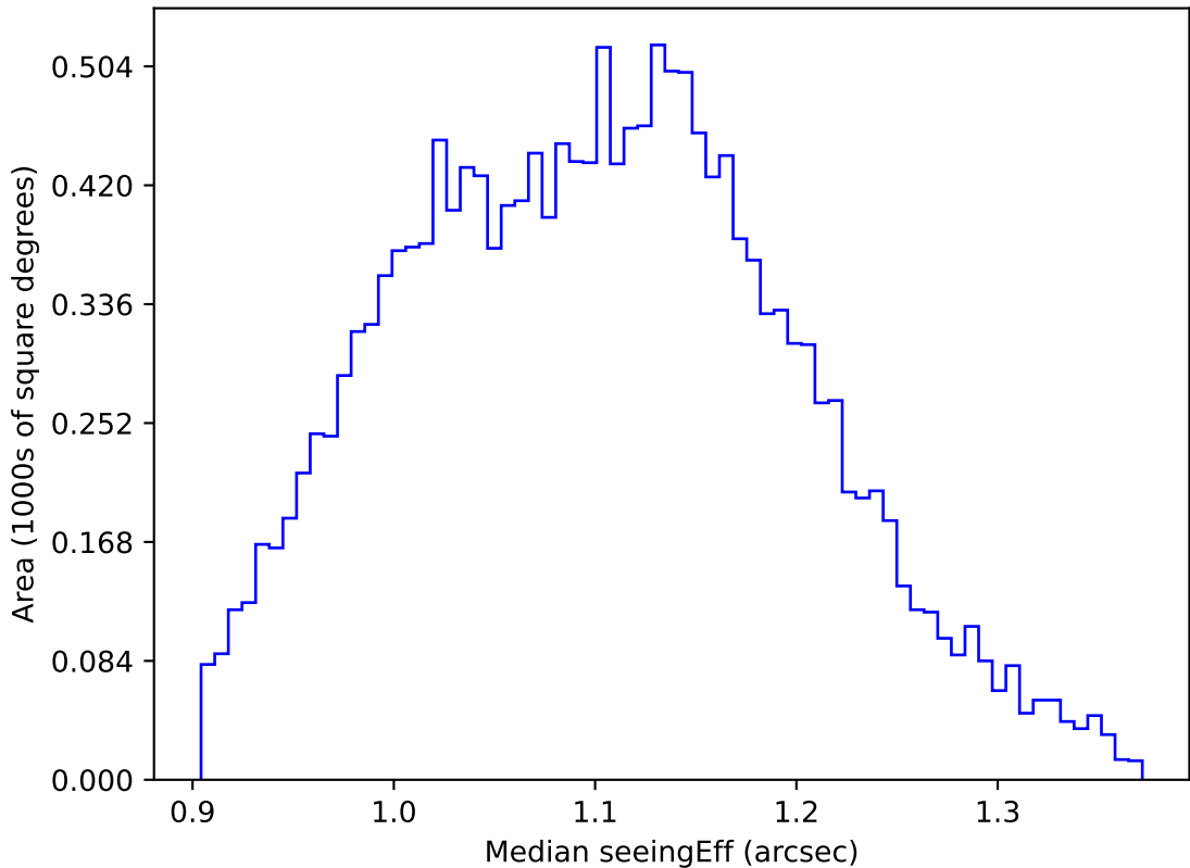
ddf_acor_sf20_lsf40_lsr50_v3.4_10yrs WFD g band: Median seeingEff
