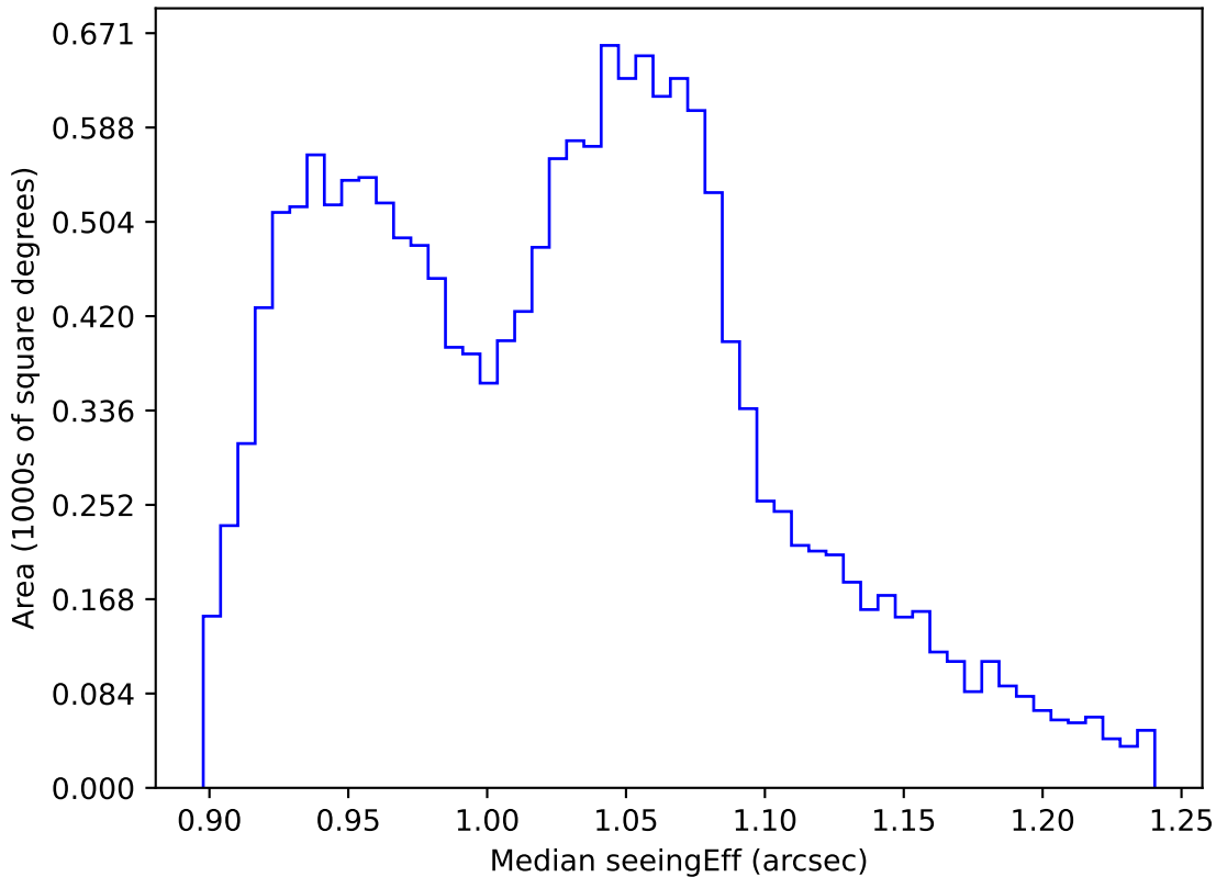
ddf_acor_sf20_lsf40_lsr50_v3.4_10yrs WFD all bands: Median seeingEff
