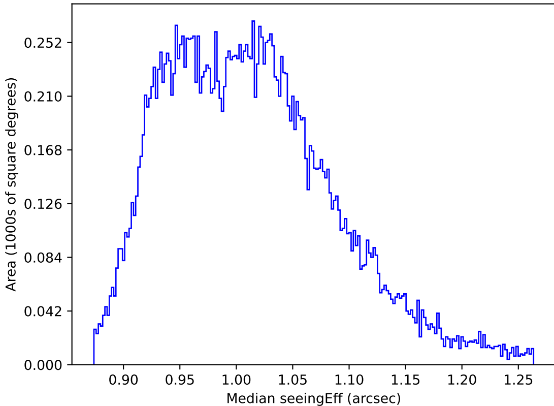
ddf_acor_sf20_lsf40_lsr50_v3.4_10yrs All sky y band: Median seeingEff
