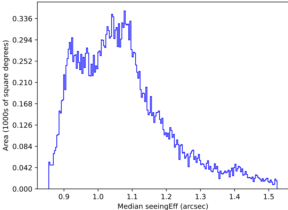
ddf_acor_sf20_lsf40_lsr50_v3.4_10yrs All sky r band: Median seeingEff
