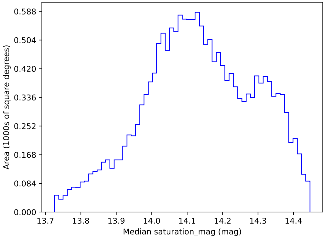
ddf_acor_sf20_lsf40_lsr50_v3.4_10yrs WFD z band: Median saturation_mag
