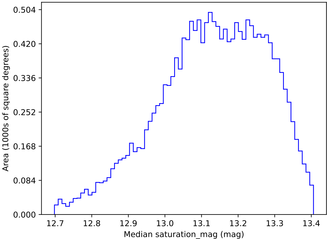
ddf_acor_sf20_lsf40_lsr50_v3.4_10yrs WFD y band: Median saturation_mag
