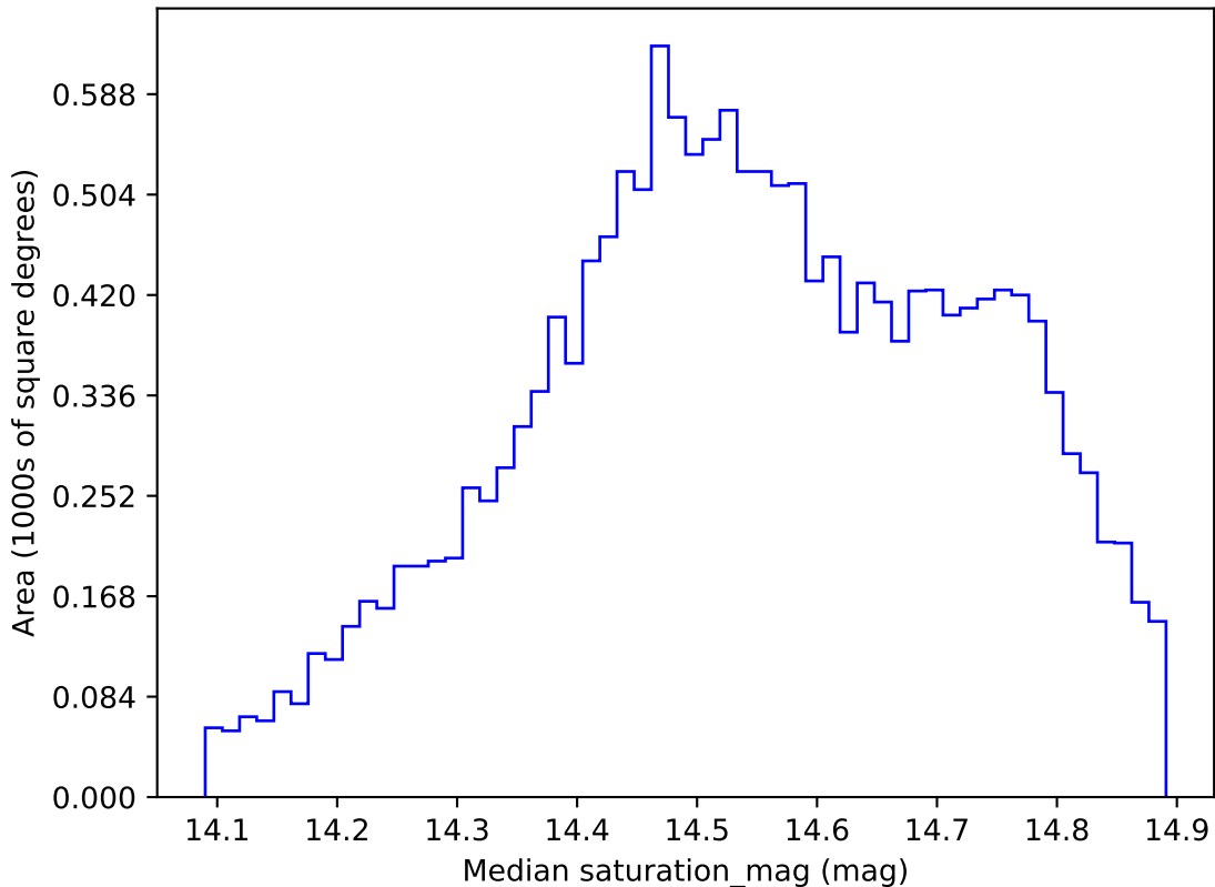
ddf_acor_sf20_lsf40_lsr50_v3.4_10yrs WFD i band: Median saturation_mag
