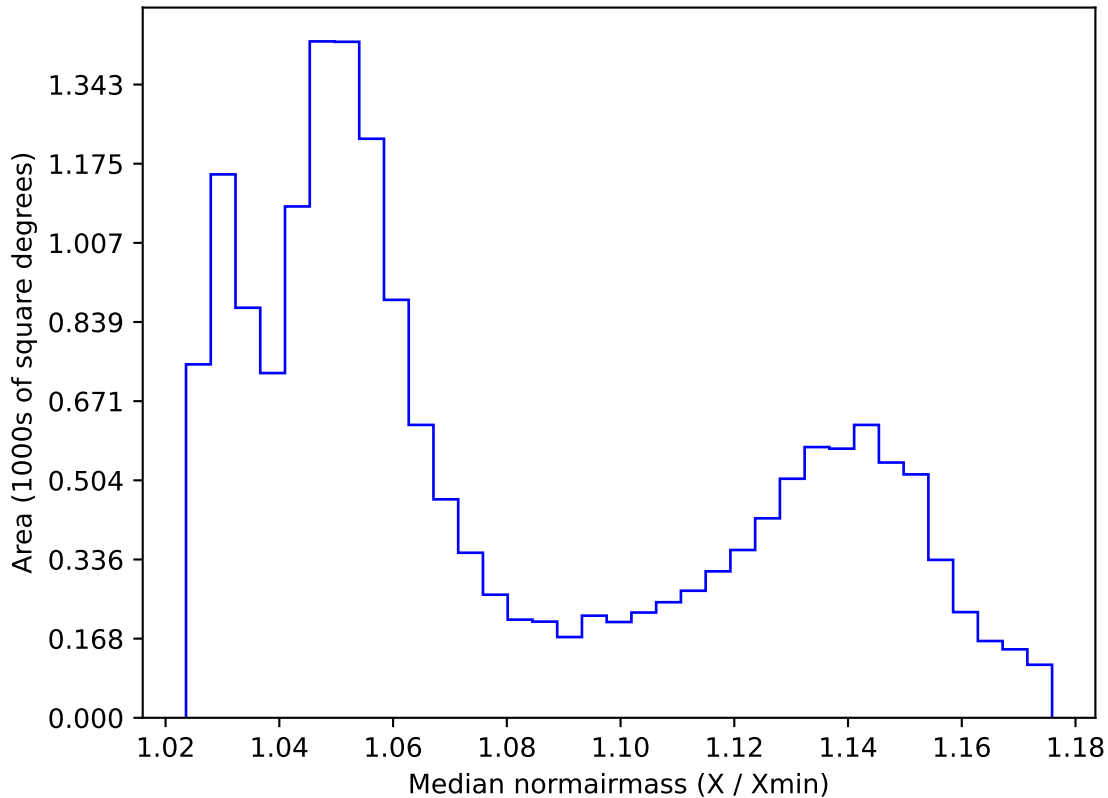
ddf_acor_sf20_lsf40_lsr50_v3.4_10yrs WFD all bands: Median normairmass
