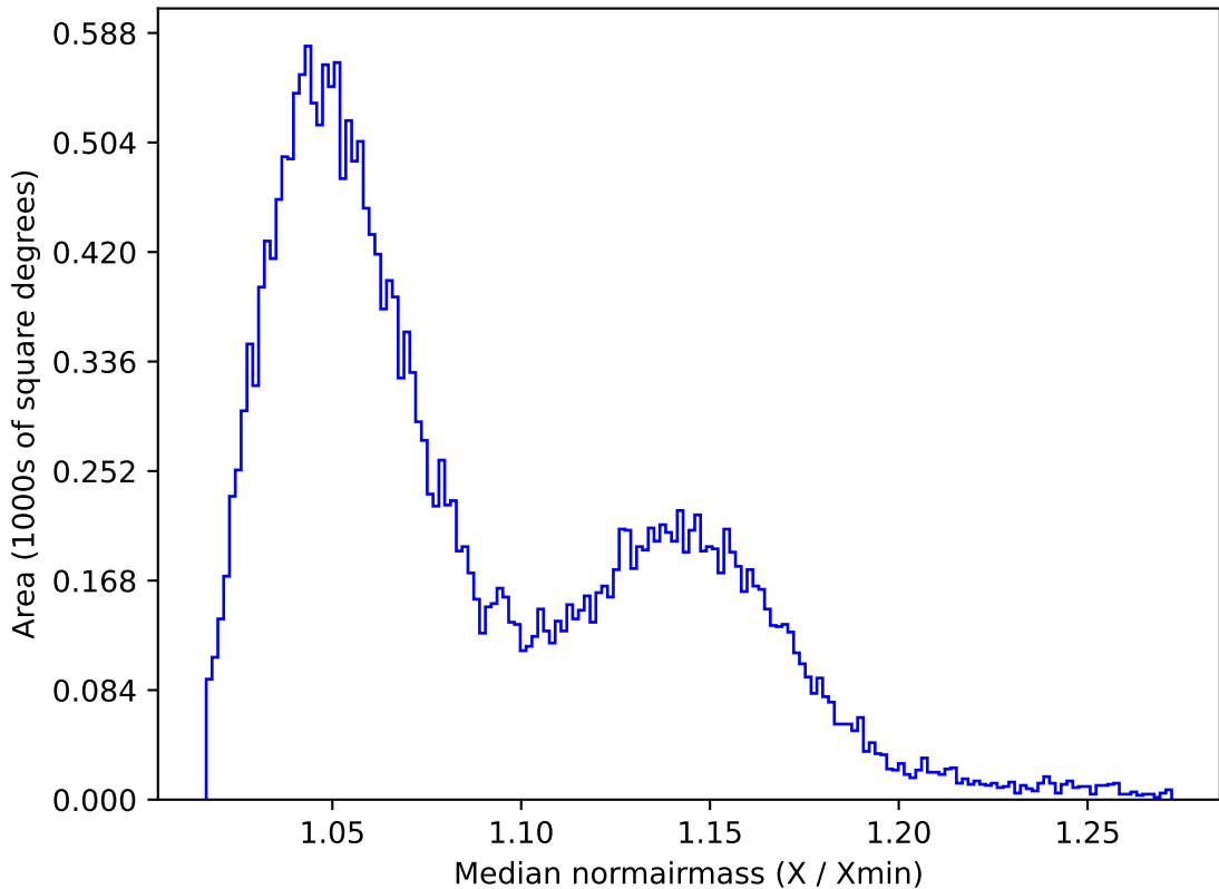
ddf_acor_sf20_lsf40_lsr50_v3.4_10yrs All sky z band: Median normairmass
