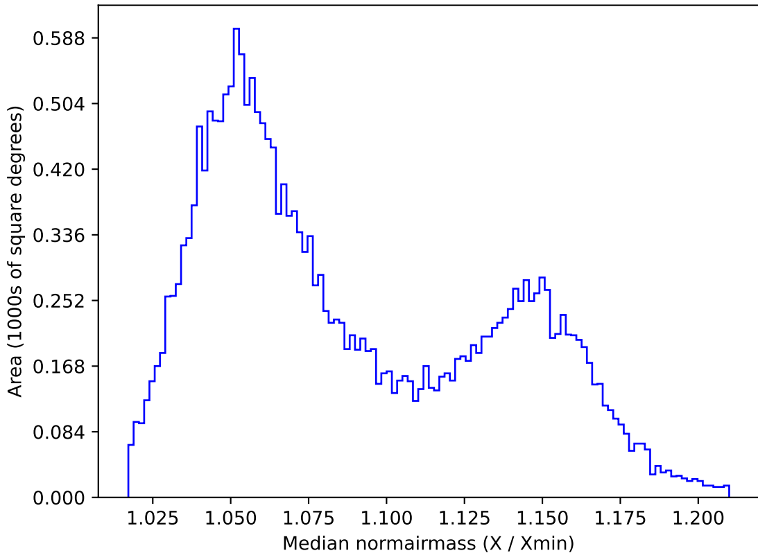
ddf_acor_sf20_lsf40_lsr50_v3.4_10yrs All sky y band: Median normairmass
