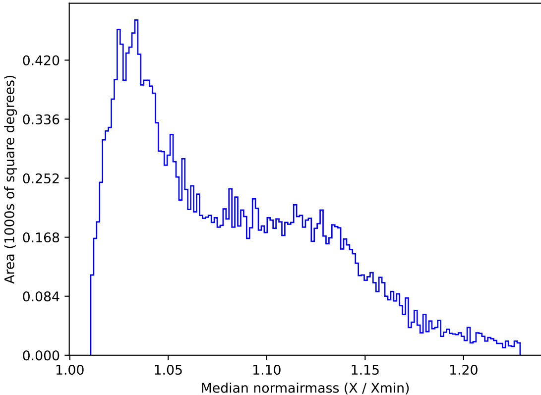
ddf_acor_sf20_lsf40_lsr50_v3.4_10yrs All sky u band: Median normairmass
