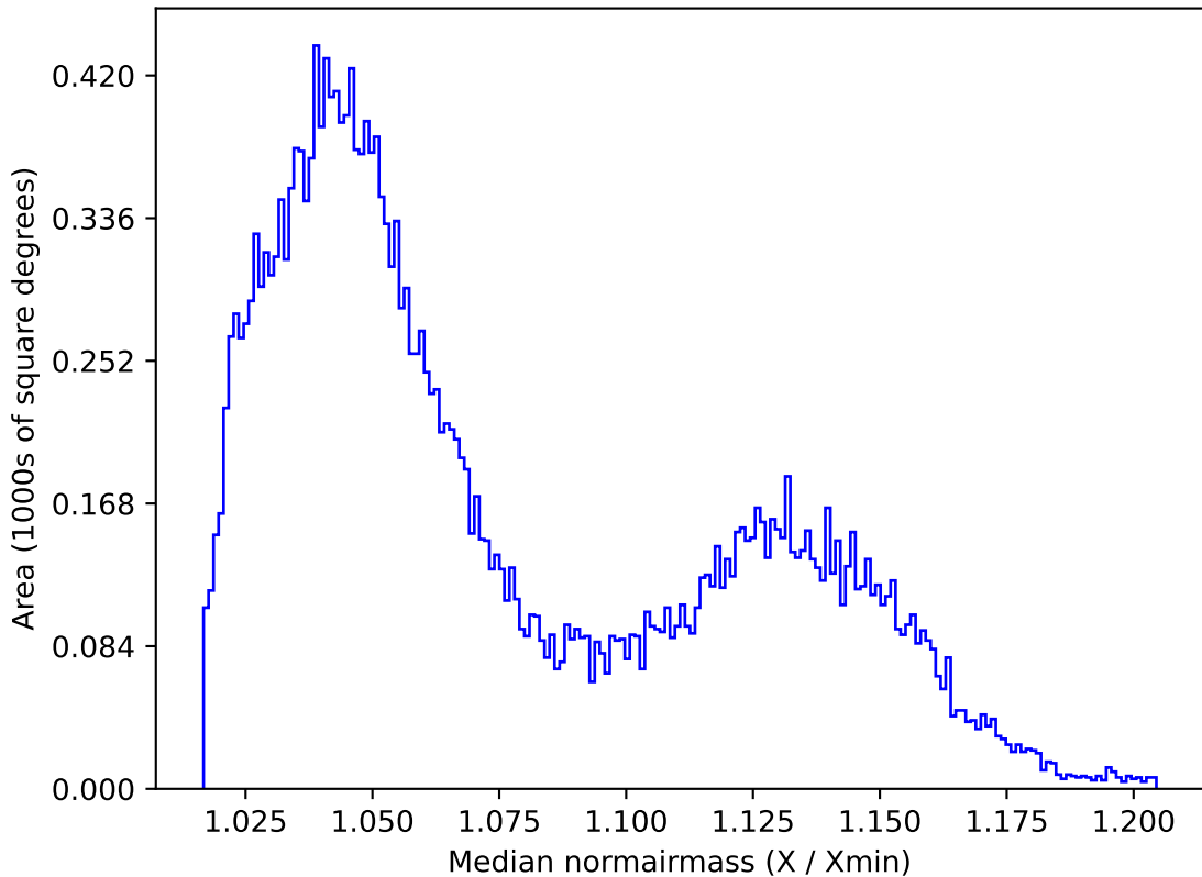
ddf_acor_sf20_lsf40_lsr50_v3.4_10yrs All sky i band: Median normairmass
