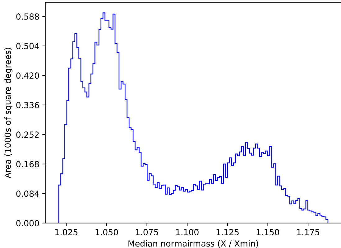
ddf_acor_sf20_lsf40_lsr50_v3.4_10yrs All sky all bands: Median normairmass
