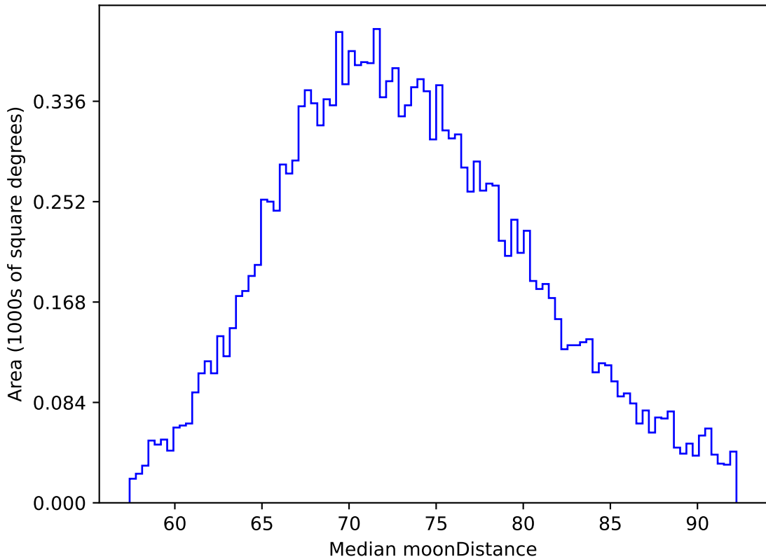
ddf_acor_sf20_lsf40_lsr50_v3.4_10yrs WFD z band: Median moonDistance
