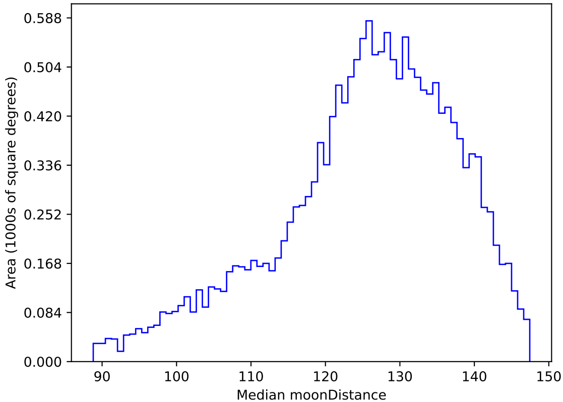
ddf_acor_sf20_lsf40_lsr50_v3.4_10yrs WFD u band: Median moonDistance
