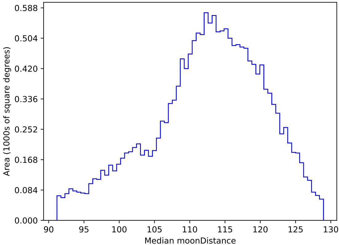
ddf_acor_sf20_lsf40_lsr50_v3.4_10yrs WFD r band: Median moonDistance
