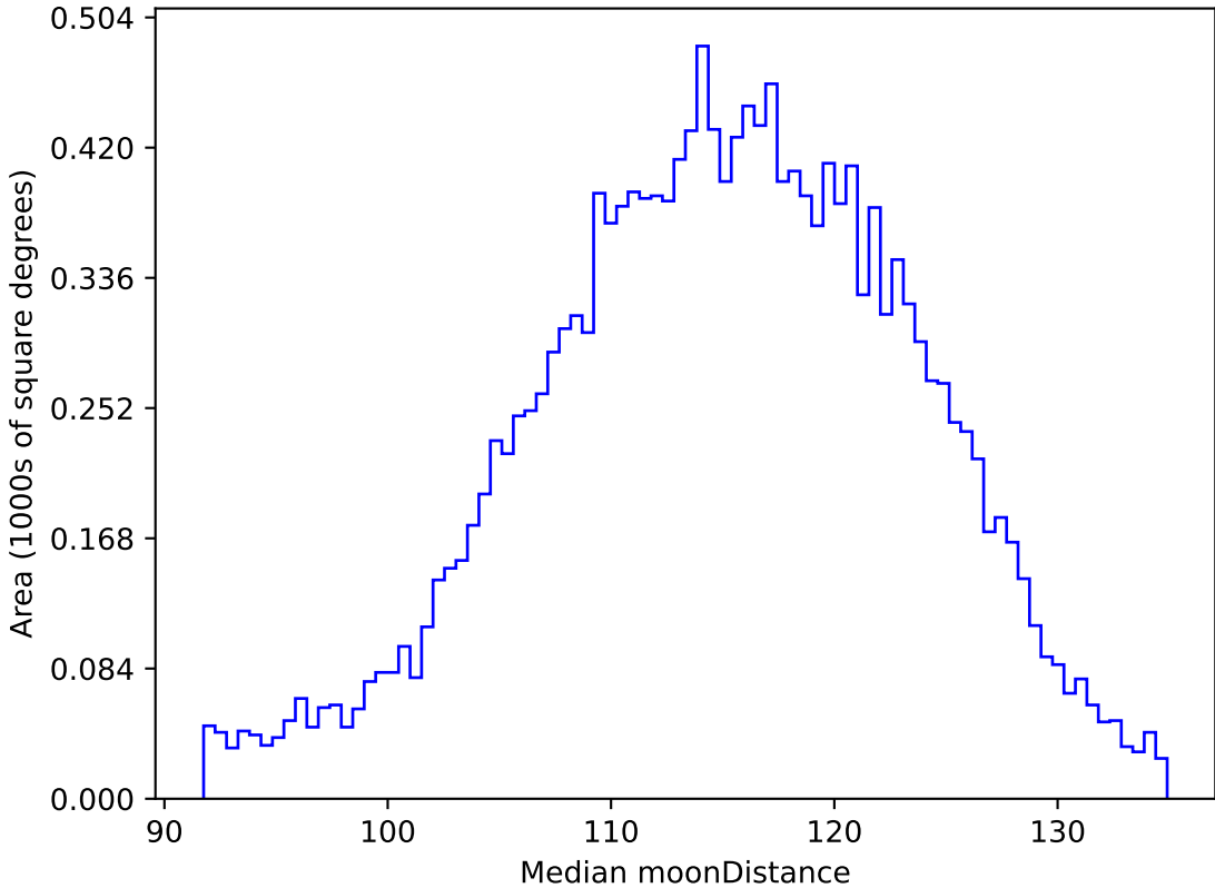
ddf_acor_sf20_lsf40_lsr50_v3.4_10yrs WFD g band: Median moonDistance
