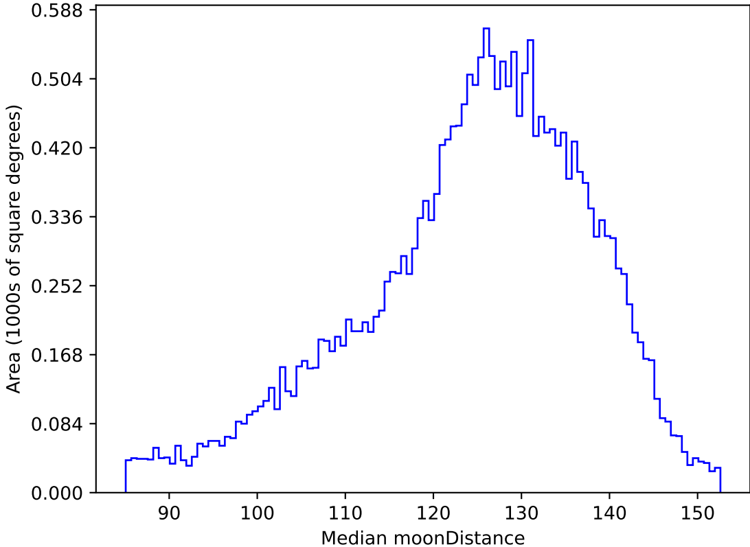
ddf_acor_sf20_lsf40_lsr50_v3.4_10yrs All sky u band: Median moonDistance
