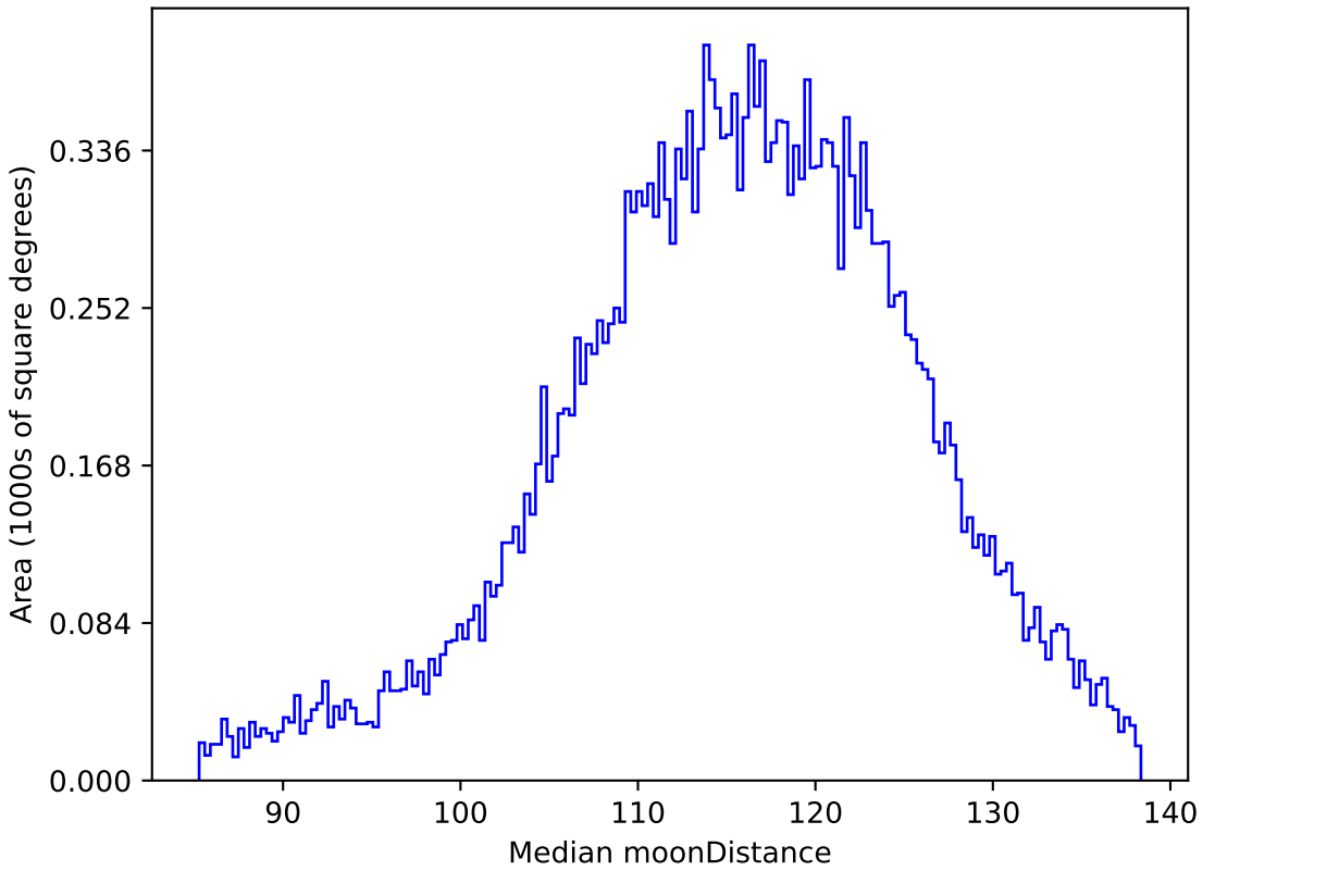
ddf_acor_sf20_lsf40_lsr50_v3.4_10yrs All sky g band: Median moonDistance
