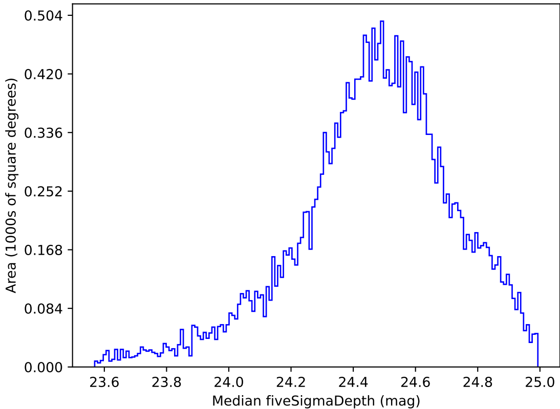
ddf_acor_sf20_lsf40_lsr50_v3.4_10yrs Yr 1 g band: Median fiveSigmaDepth
