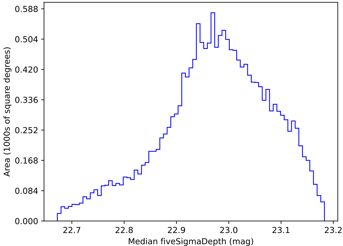
ddf_acor_sf20_lsf40_lsr50_v3.4_10yrs WFD z band: Median fiveSigmaDepth
