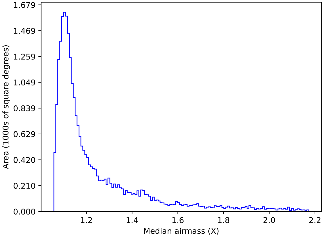
ddf_acor_sf20_lsf40_lsr50_v3.4_10yrs Yr 1 i band: Median airmass
