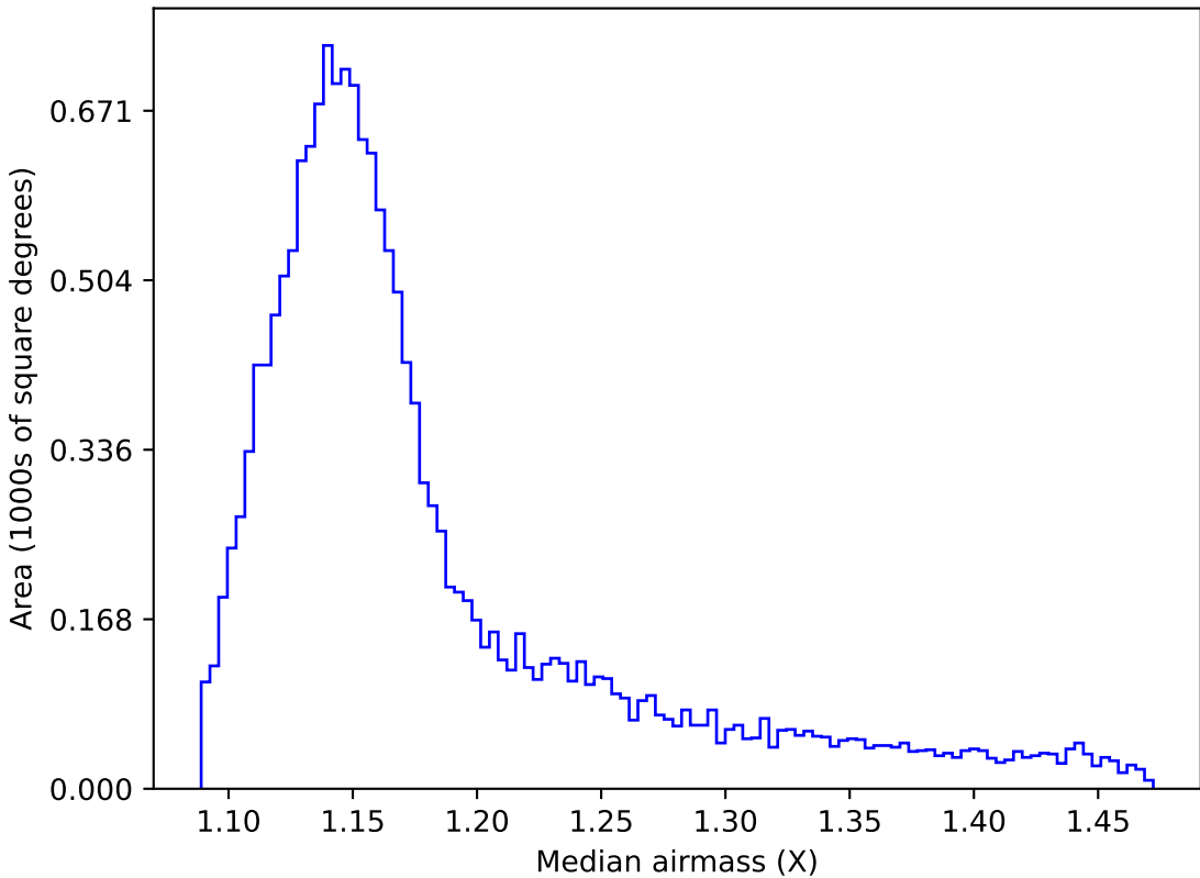
ddf_acor_sf20_lsf40_lsr50_v3.4_10yrs WFD z band: Median airmass
