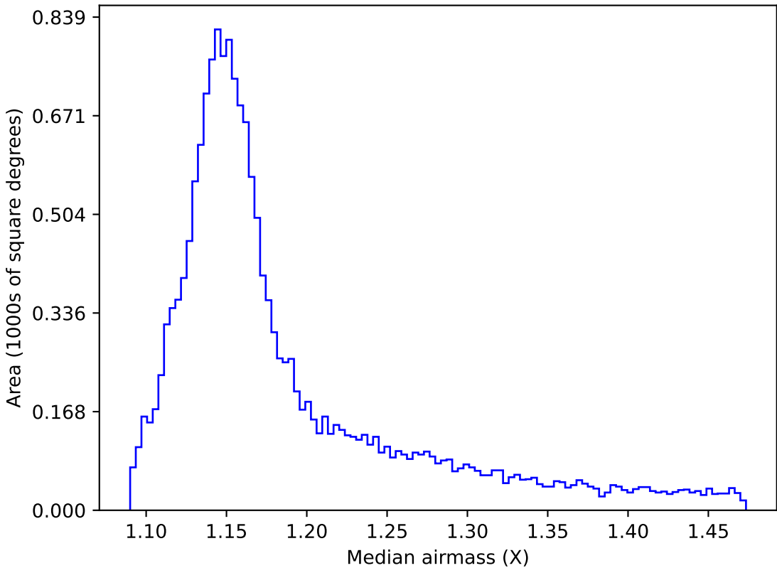
ddf_acor_sf20_lsf40_lsr50_v3.4_10yrs WFD y band: Median airmass
