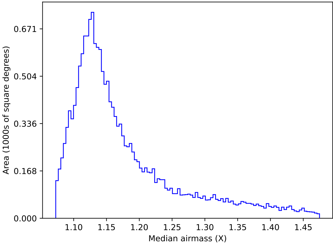
ddf_acor_sf20_lsf40_lsr50_v3.4_10yrs WFD u band: Median airmass
