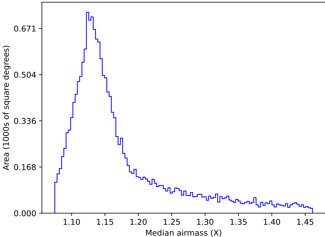
ddf_acor_sf20_lsf40_lsr50_v3.4_10yrs WFD r band: Median airmass
