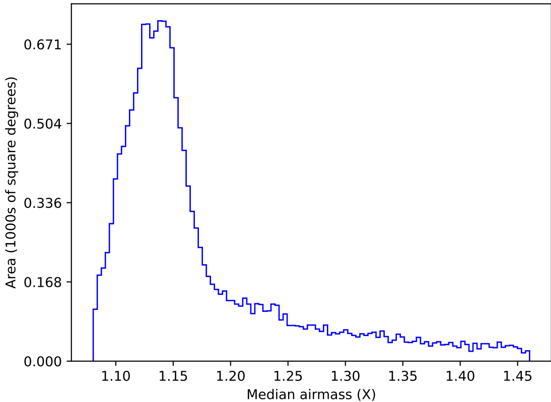
ddf_acor_sf20_lsf40_lsr50_v3.4_10yrs WFD i band: Median airmass
