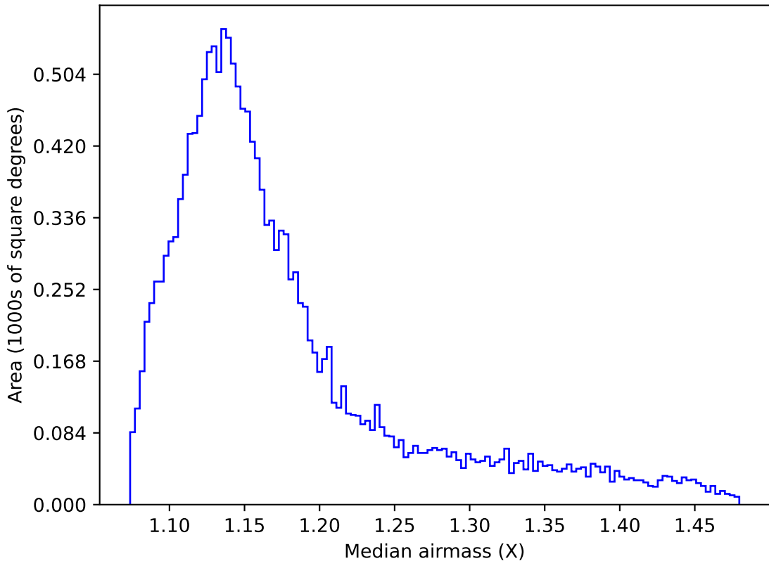
ddf_acor_sf20_lsf40_lsr50_v3.4_10yrs WFD g band: Median airmass
