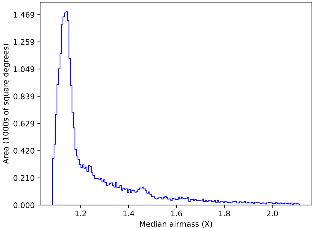
ddf_acor_sf20_lsf40_lsr50_v3.4_10yrs All sky i band: Median airmass
