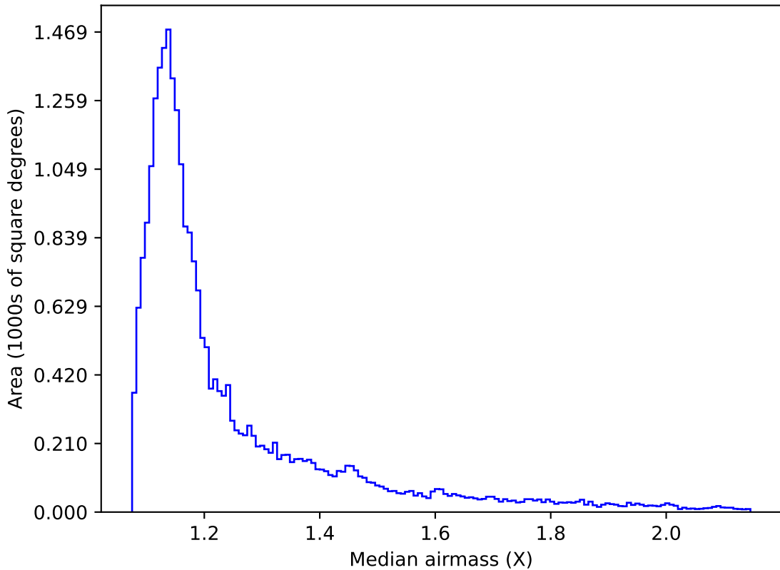
ddf_acor_sf20_lsf40_lsr50_v3.4_10yrs All sky g band: Median airmass
