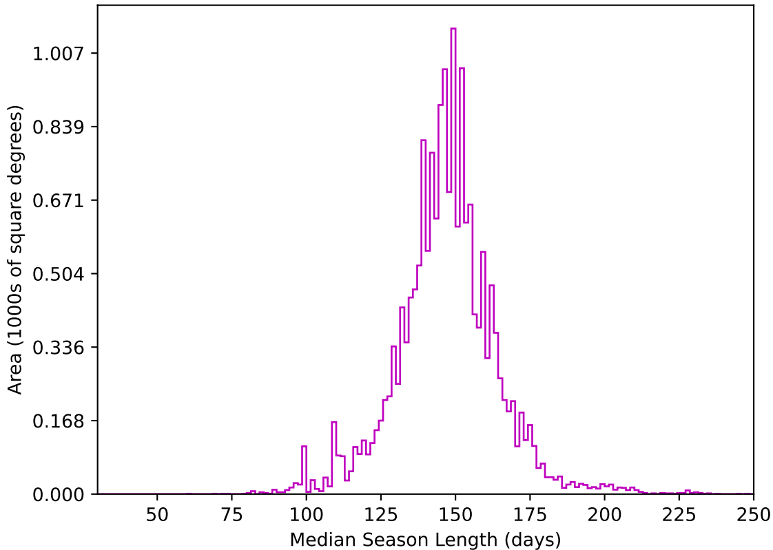
ddf_acor_sf20_lsf40_lsr50_v3.4_10yrs WFD z band: Median Season Length
