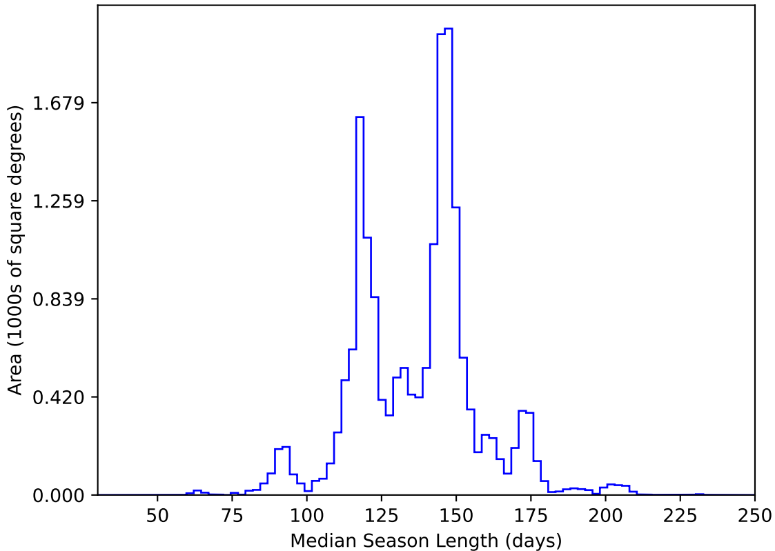
ddf_acor_sf20_lsf40_lsr50_v3.4_10yrs WFD y band: Median Season Length
