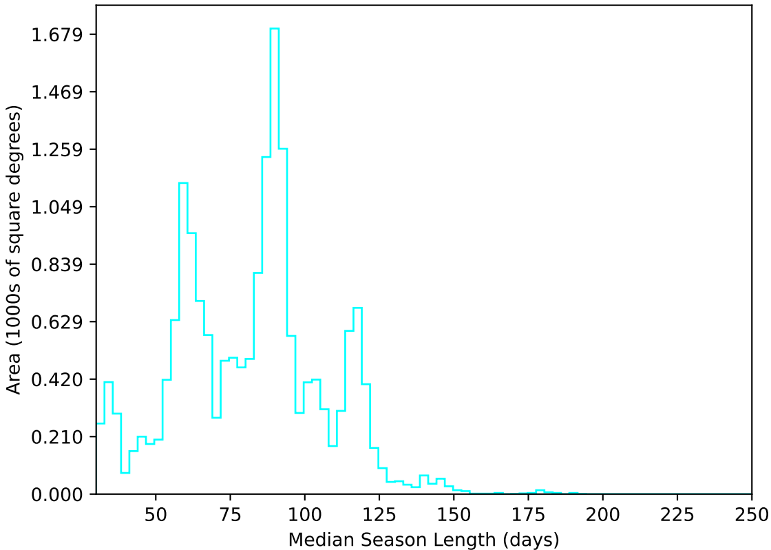
ddf_acor_sf20_lsf40_lsr50_v3.4_10yrs WFD u band: Median Season Length
