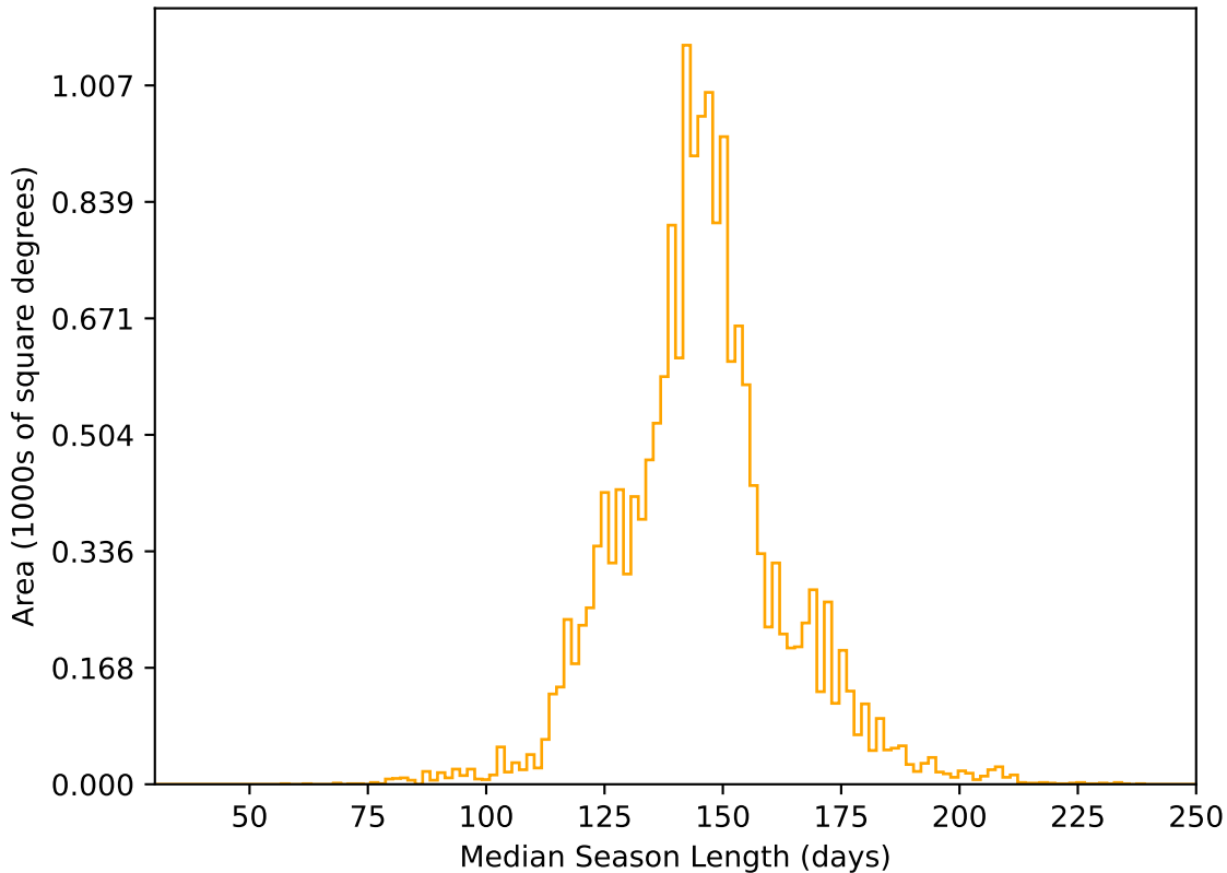
ddf_acor_sf20_lsf40_lsr50_v3.4_10yrs WFD r band: Median Season Length
