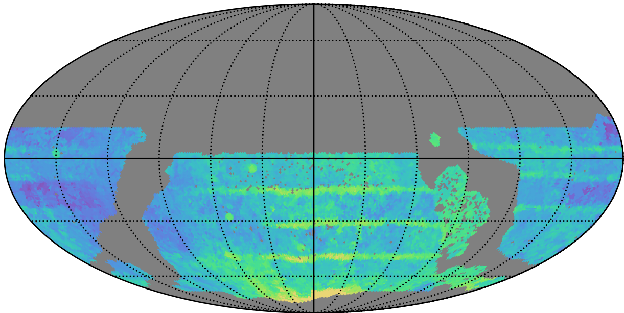
ddf_acor_sf20_lsf40_lsr50_v3.4_10yrs WFD all bands: Median Season Length
