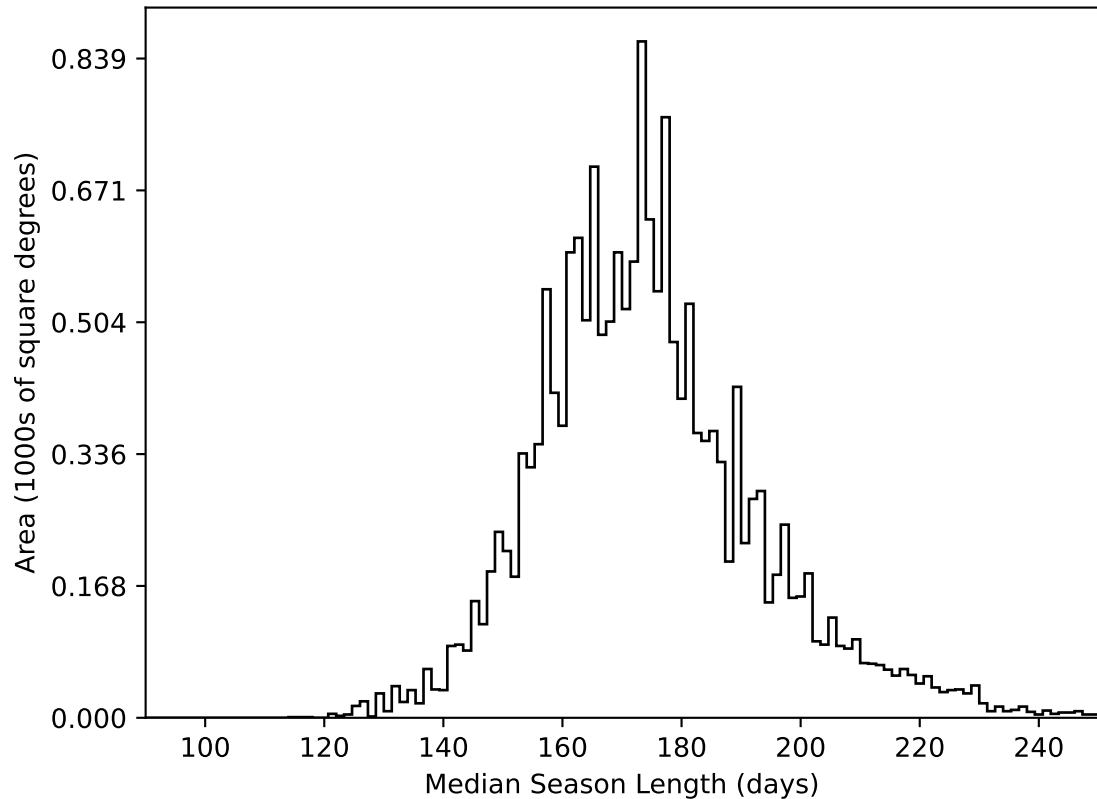
ddf_acor_sf20_lsf40_lsr50_v3.4_10yrs WFD all bands: Median Season Length
