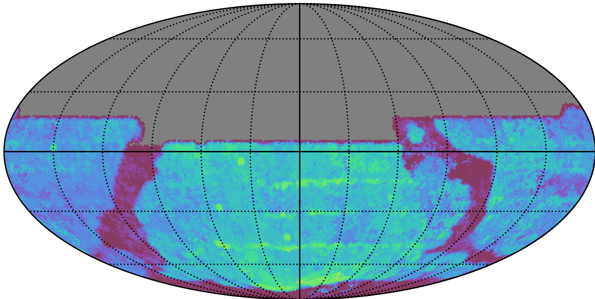
ddf_acor_sf20_lsf40_lsr50_v3.4_10yrs All sky y band: Median Season Length
