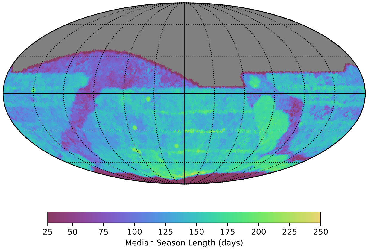
ddf_acor_sf20_lsf40_lsr50_v3.4_10yrs All sky r band: Median Season Length
