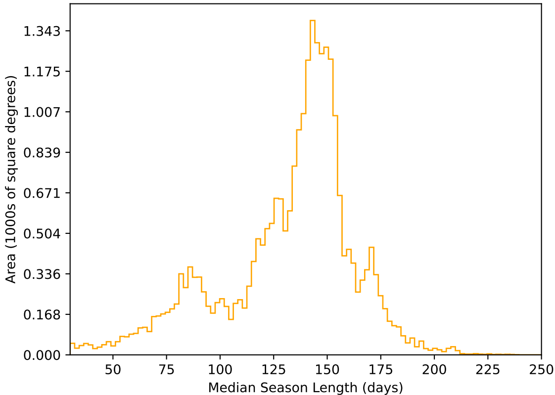
ddf_acor_sf20_lsf40_lsr50_v3.4_10yrs All sky r band: Median Season Length
