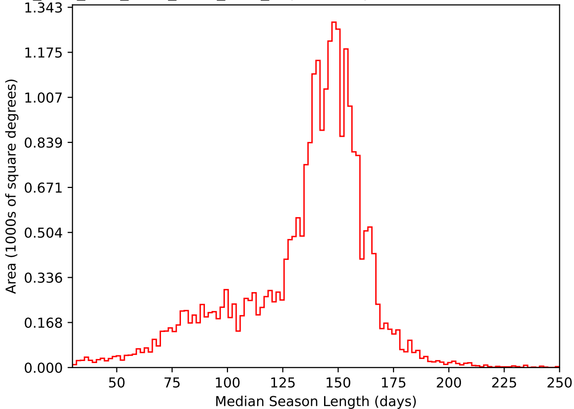
ddf_acor_sf20_lsf40_lsr50_v3.4_10yrs All sky i band: Median Season Length
