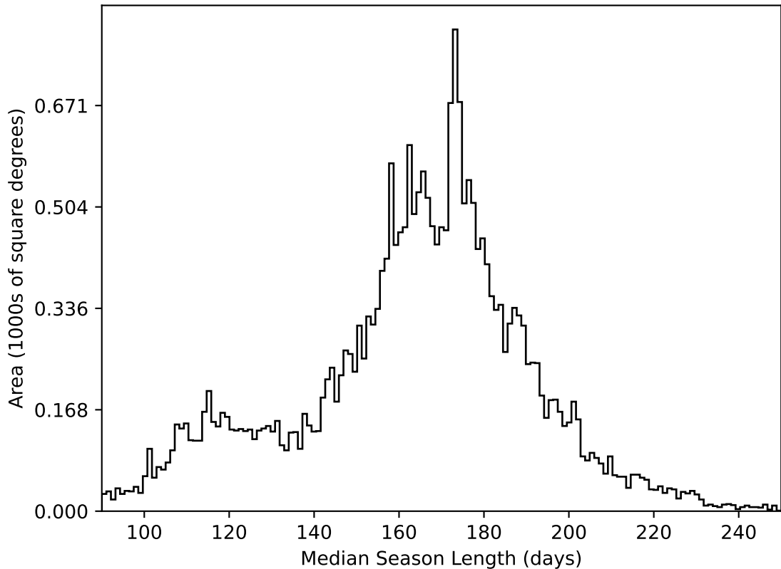
ddf_acor_sf20_lsf40_lsr50_v3.4_10yrs All sky all bands: Median Season Length
