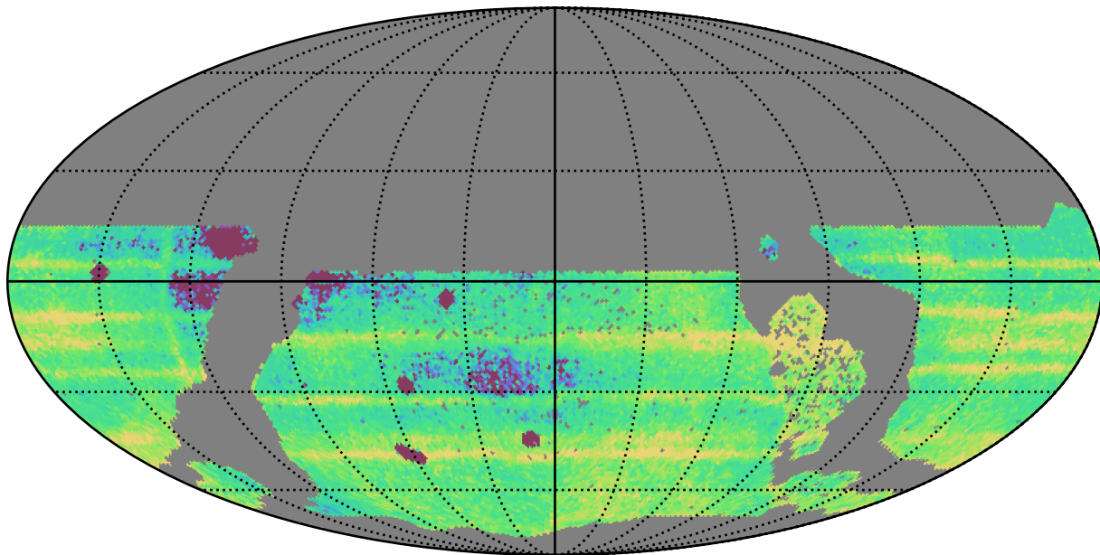
ddf_acor_sf20_lsf40_lsr50_v3.4_10yrs WFD: Median Intra-Night Gap
