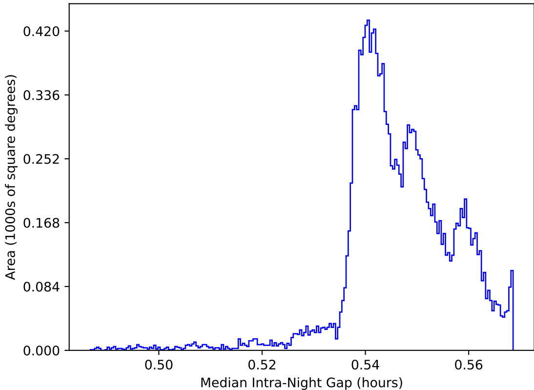
ddf_acor_sf20_lsf40_lsr50_v3.4_10yrs WFD: Median Intra-Night Gap
