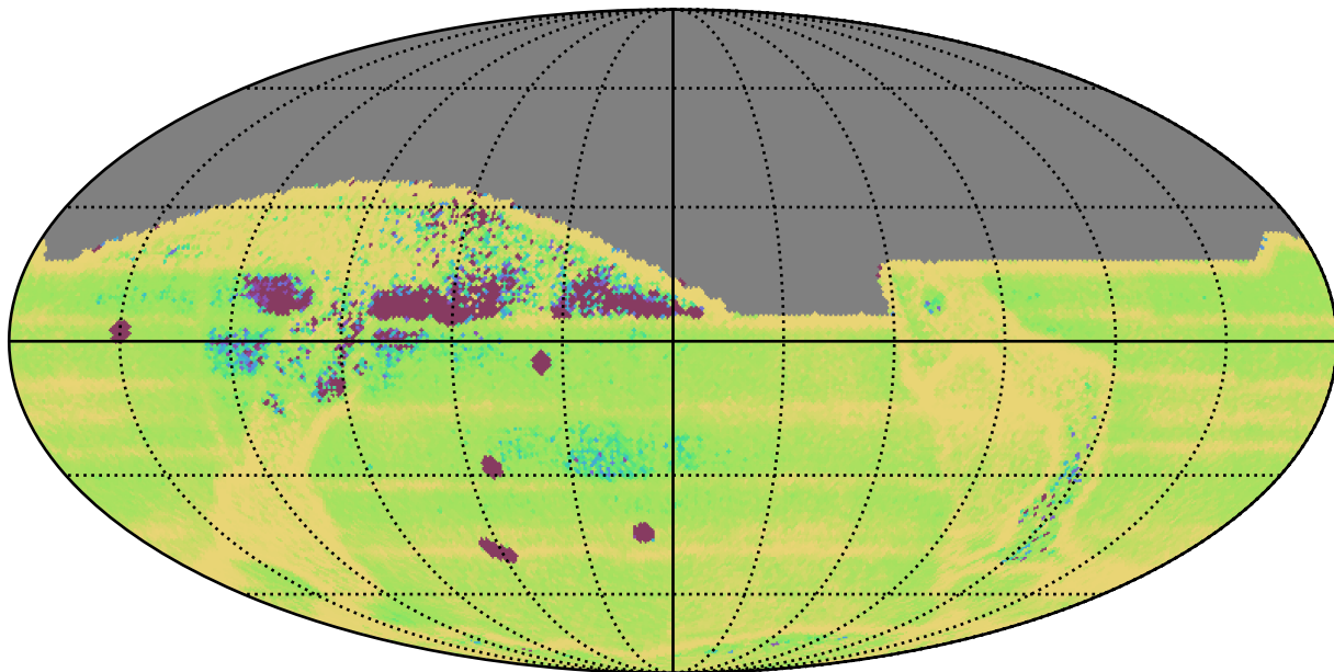
ddf_acor_sf20_lsf40_lsr50_v3.4_10yrs All sky: Median Intra-Night Gap
