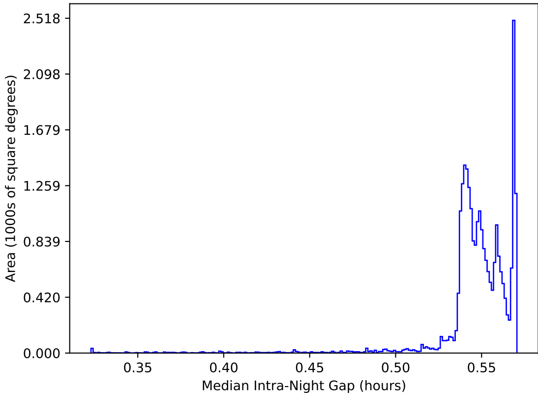
ddf_acor_sf20_lsf40_lsr50_v3.4_10yrs All sky: Median Intra-Night Gap
