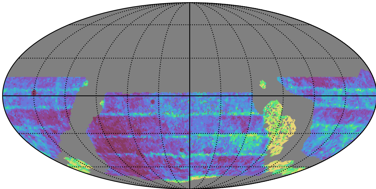
ddf_acor_sf20_lsf40_lsr50_v3.4_10yrs WFD z band: Median Inter-Night Gap
