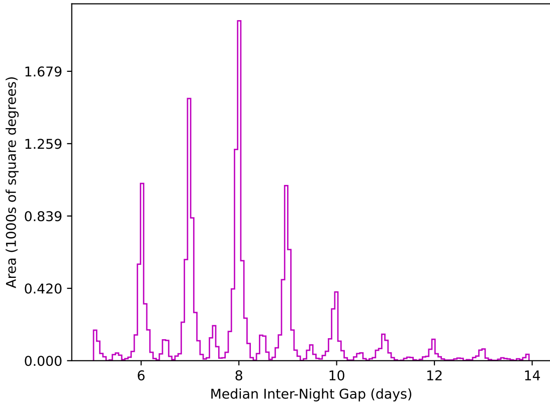
ddf_acor_sf20_lsf40_lsr50_v3.4_10yrs WFD z band: Median Inter-Night Gap
